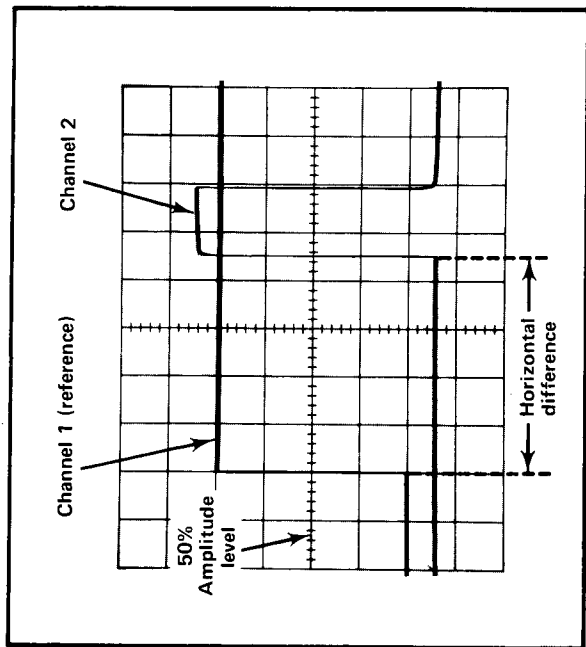
Fig. 6. Measuring time difference between two pulses.
