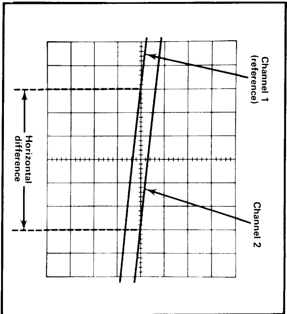
Fig. 10. High-resolution phase-difference measurement with increased sweep rate.
